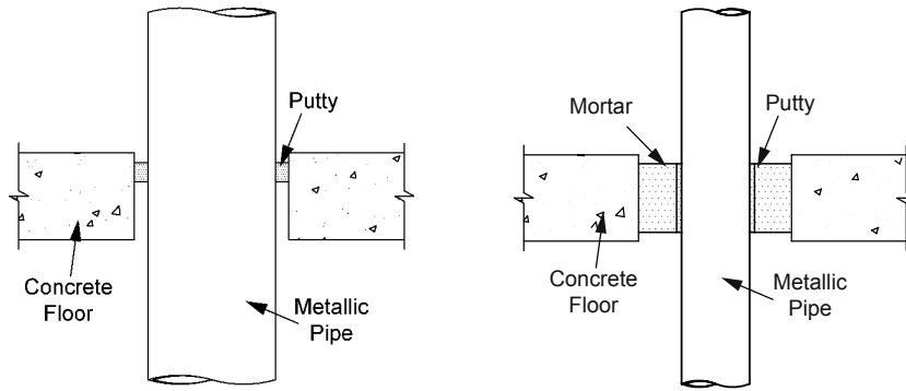
Fig. 1: METALLIC PIPE PENETRATIONS - CONCRETE/MASONRY FLOOR
