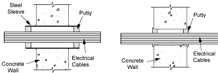
Fig. 2: METALLIC PIPE PENETRATIONS - WALLS
