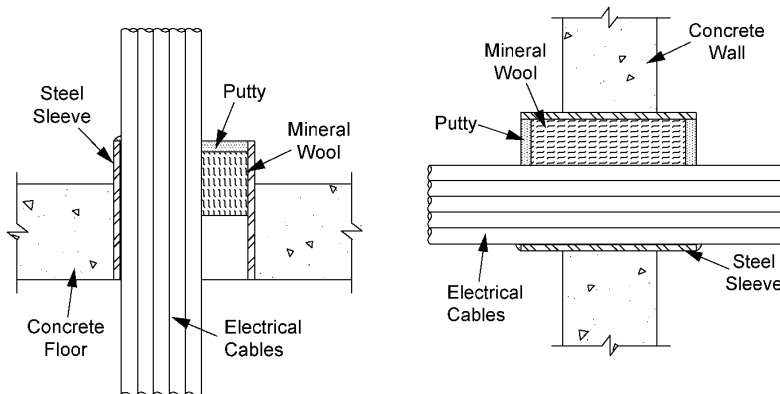
Fig. 3: CABLE PENETRATIONS - CONCRETE/MASONRY FLOORS & WALLS
